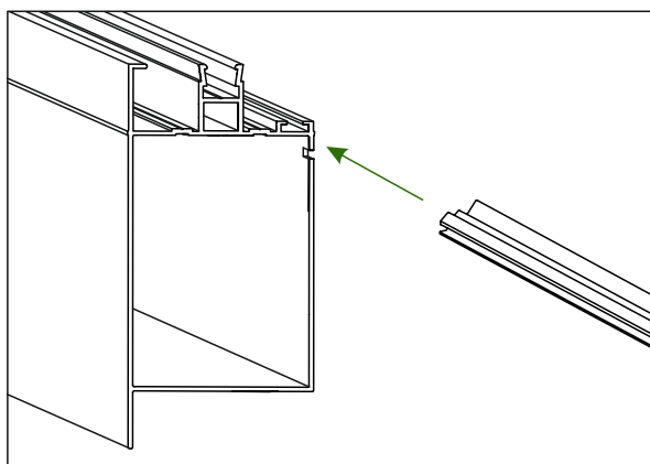
Randsparren
