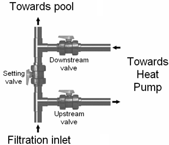
By-pass diagram
