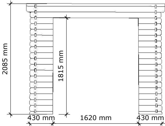
Wand A
