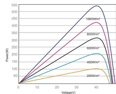
P-V Curves (545W)
