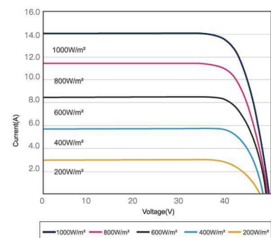
I-V Curves (545W)
