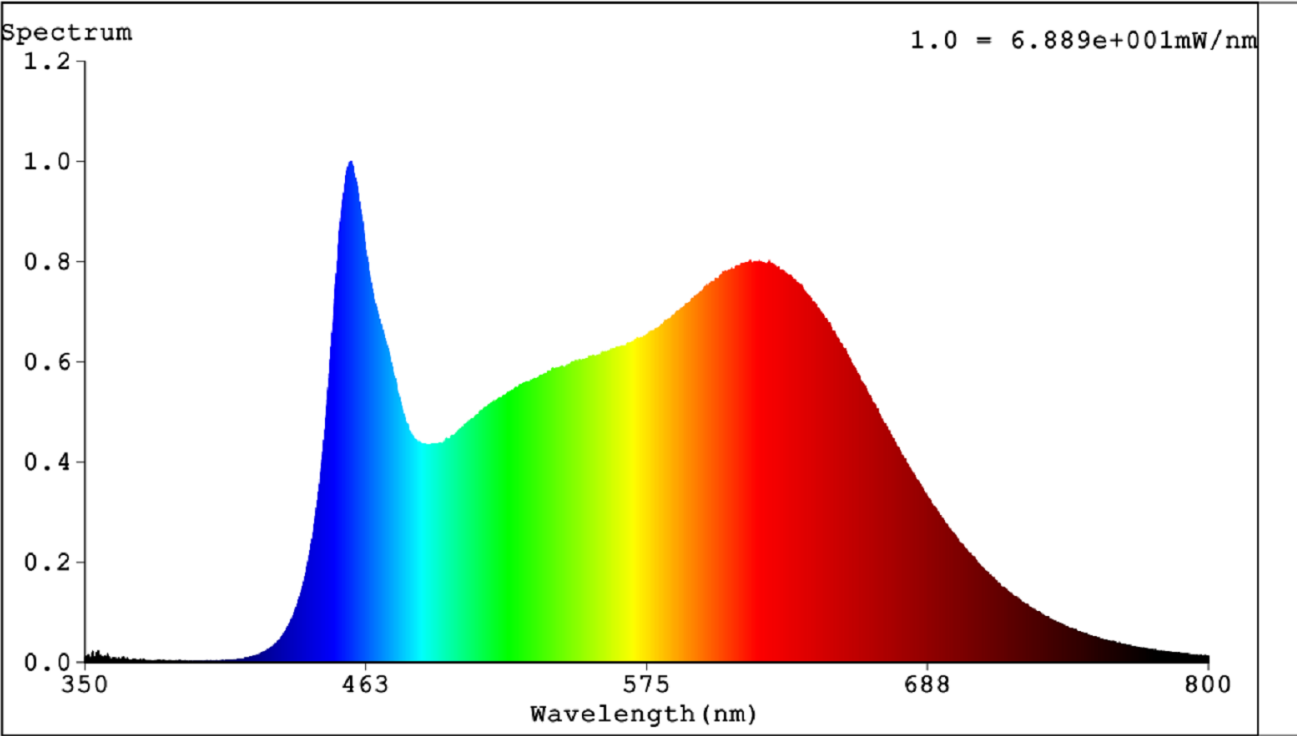
Spectral Distribution
