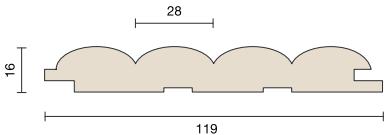
Lamelle Wave | Lamella Wave 2750x119x16 mm
