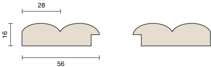
Start- und Endlamelle Wave | Start and End Lamella Wave 2750x56x16 mm
