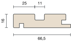
Startlamelle Beats | Start Lamella Beats 2750x66,5x16 mm
