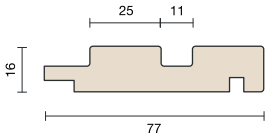
Endlamelle Beats | End Lamella Beats 2750x77x16 mm
