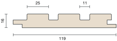
Lamelle Beats | Lamella Beats 2750x119x16 mm
