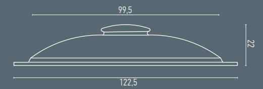
DM 506 ED: 122,5 cm ID: 99,5 cm D: 22 cm Fibre Reinforced Plastic (FRP)
