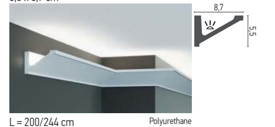
L = 200/244 cm Polyurethane
