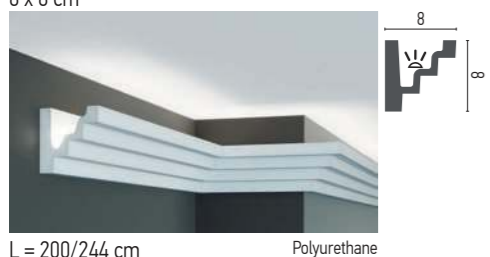
L = 200/244 cm Polyurethane
