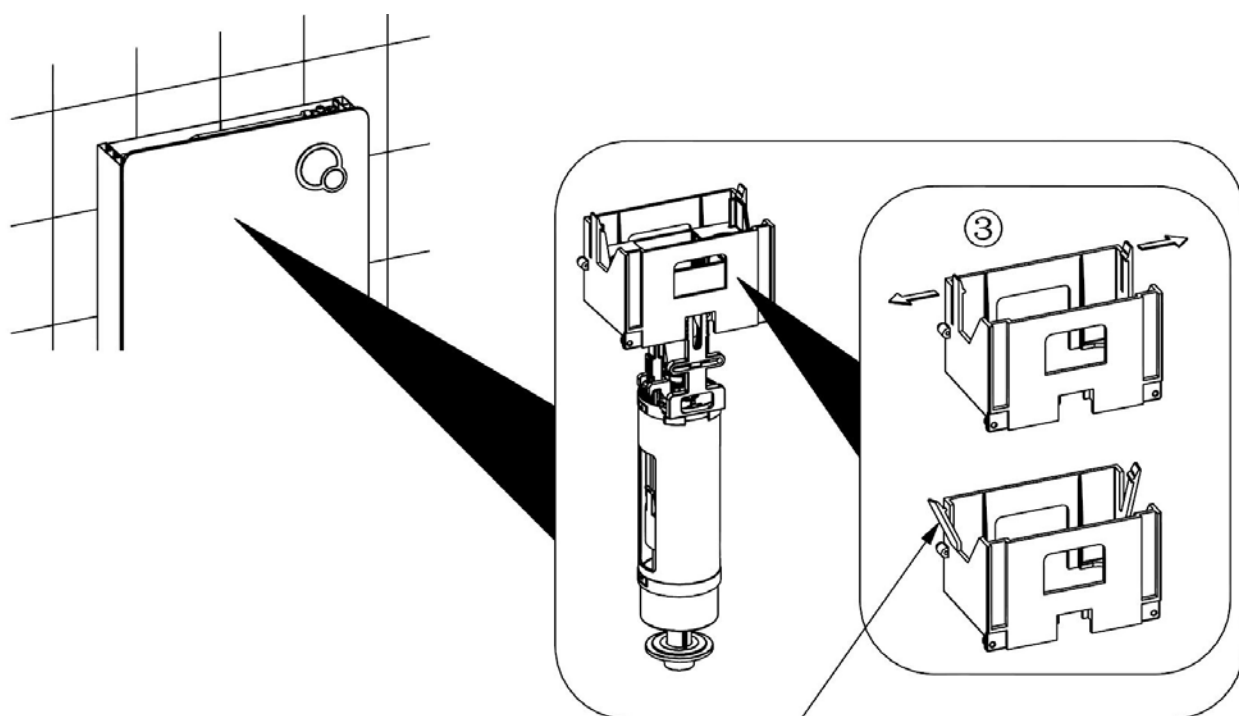
Clamps of the suspension device.
