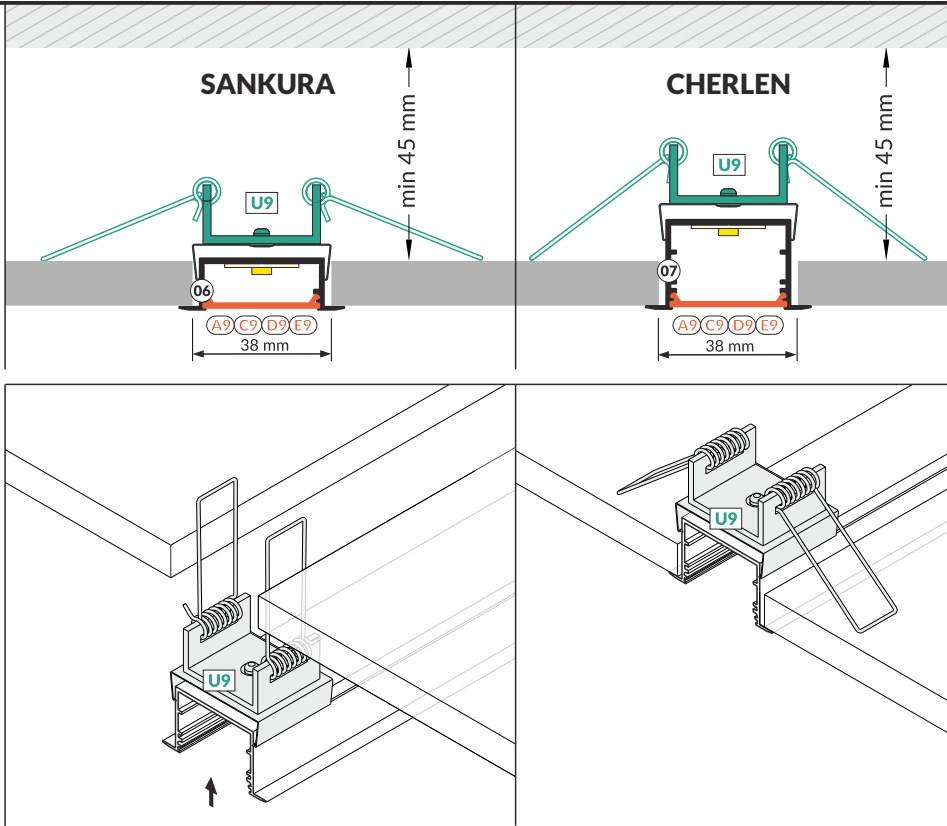
spring U9 mounting plate
