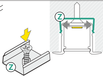
Z flexible mounting plate
