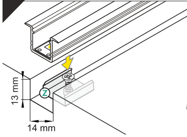
Z flexible mounting plate
