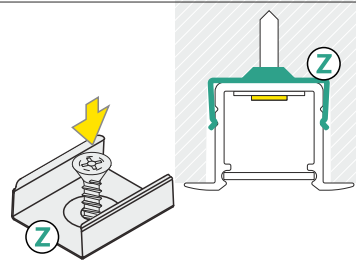
cone Z flexible mounting plate
